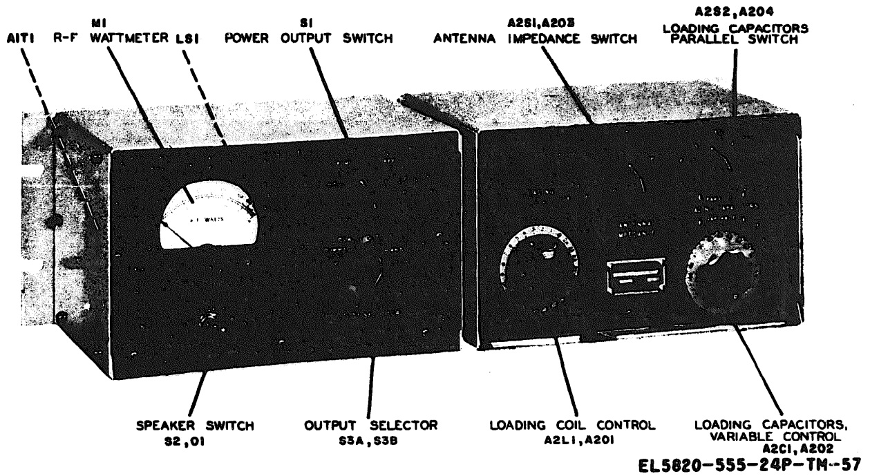
Figure 3-57. Antenna Network 180U-2, operating controls (1A2).
