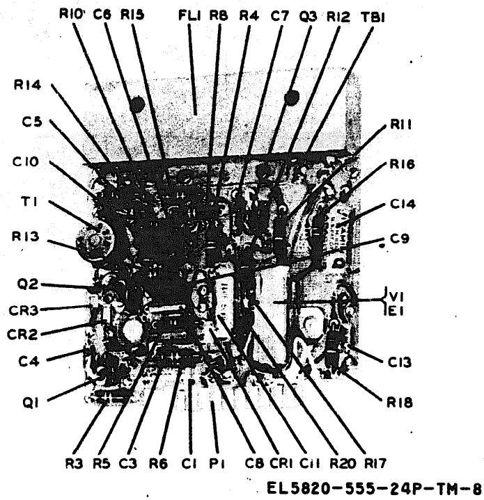
Figure 3-8. Stabilized master oscillator module, 4-kc spectrum generator assembly (1A4A3A6).
