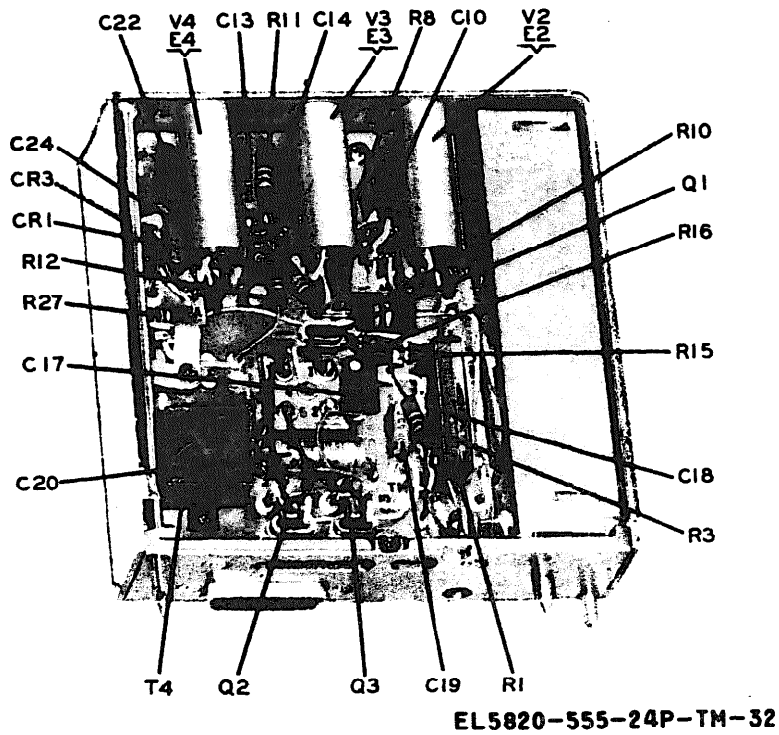
Figure 3-32. AM i-fla-f amplifier module, rear view, cover removed (1A5A6).
