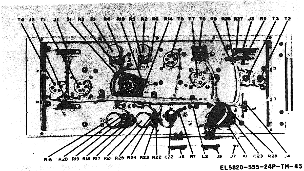
Figure 3-43. Audio and Control Unit 159B-1 chassis, rear view (1A7).
