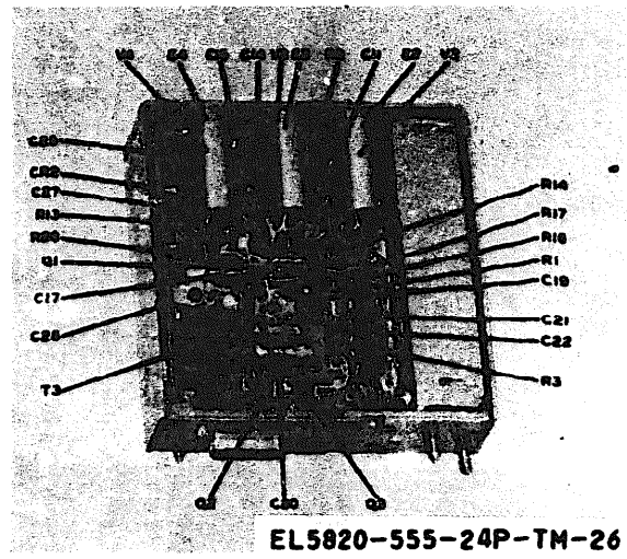
Figure 3-26. USB i-fla-f amplifier module, rear view, cover removed (1A5A4).
