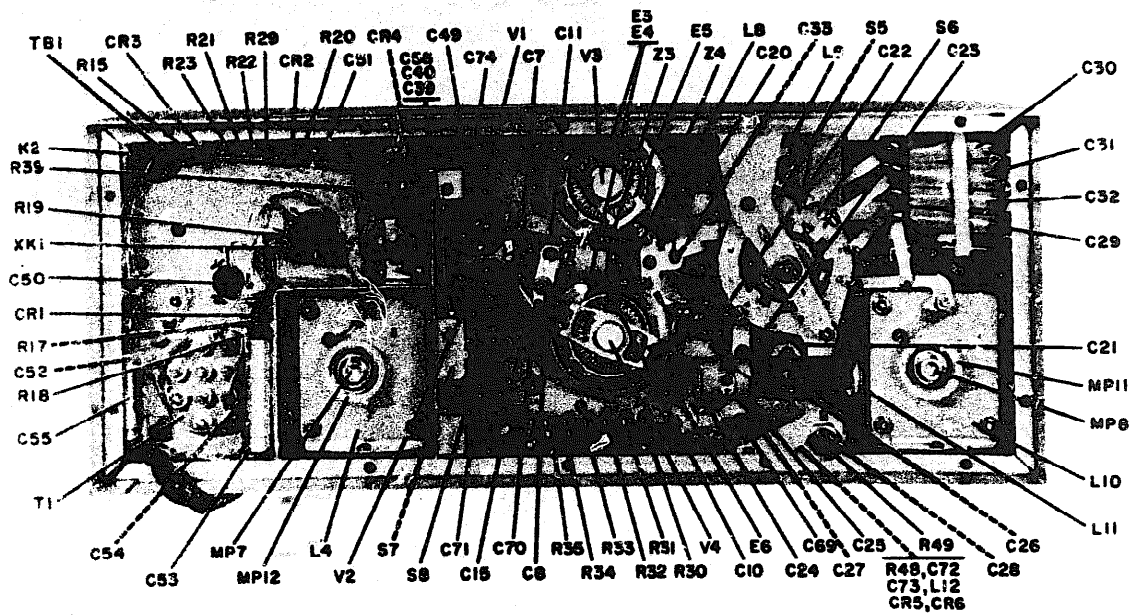
Figure 3-37. Power Amplifier 367A-3, front view, front panel removed (1A3).
