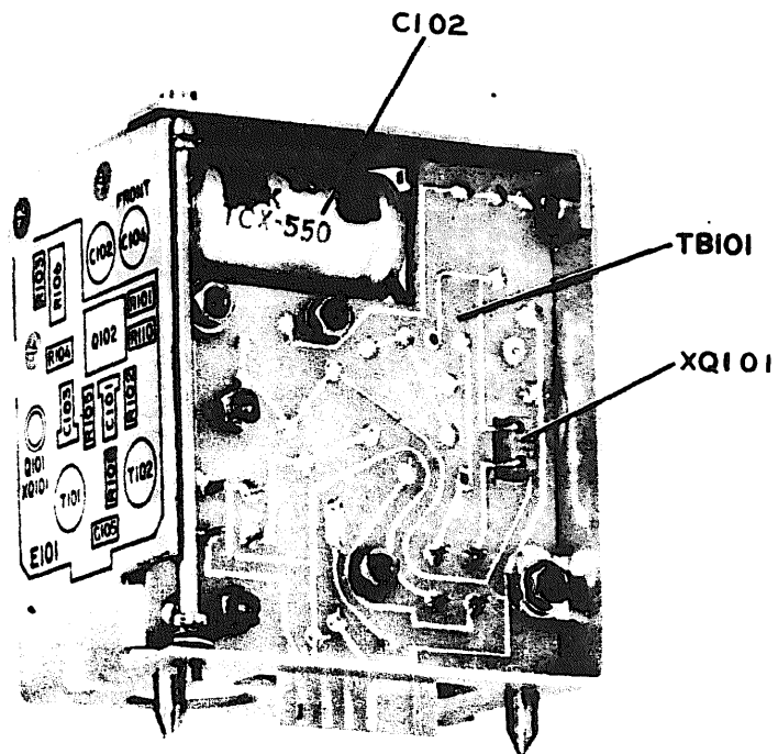
Figure 3-41. Mike or line amplifier module, wiring side (1A7A1, 1A7A2, and 1A7A3).
