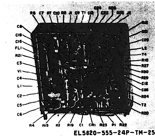
Figure 3-25. USB i-fla-f amplifier module, front view, cover removed (1A5A4).
