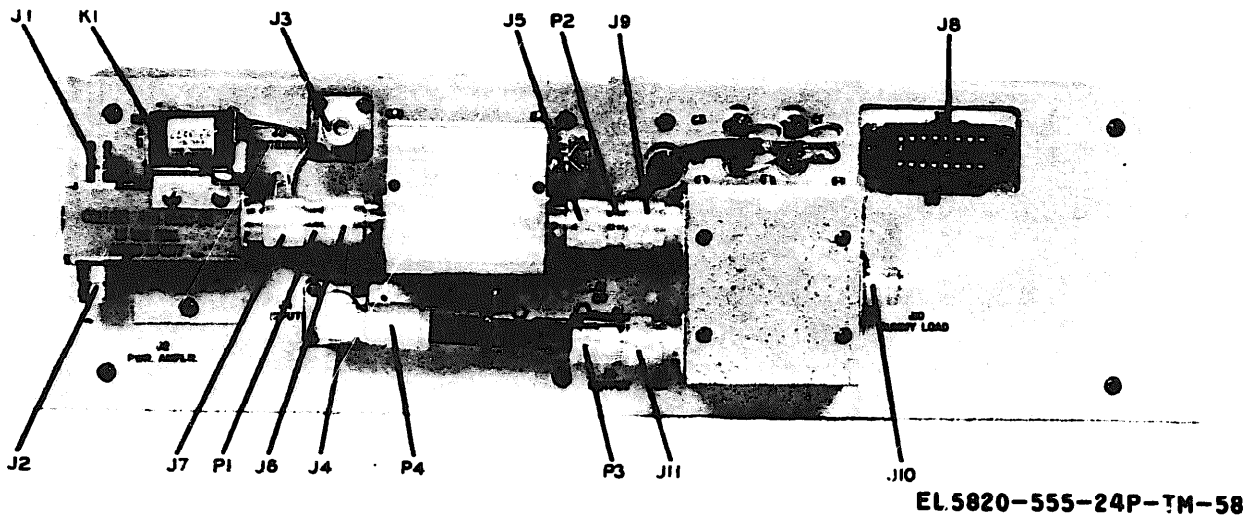
Figure 3-58. Antenna Network 180U-2, input and output connectors (1A2).
