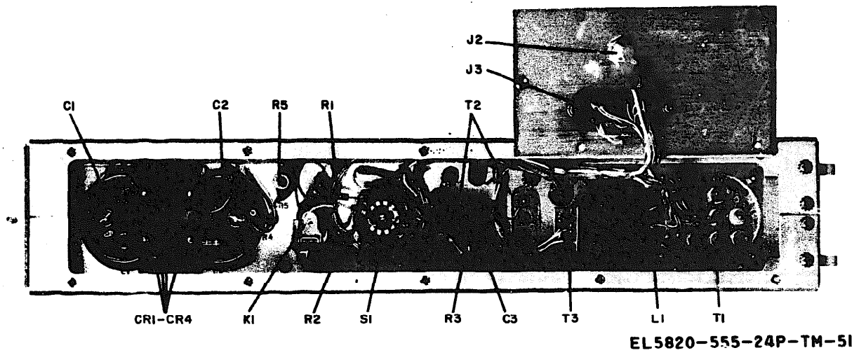
Figure 3-51. Handset adapter, rear view, cover removed (1A9).
