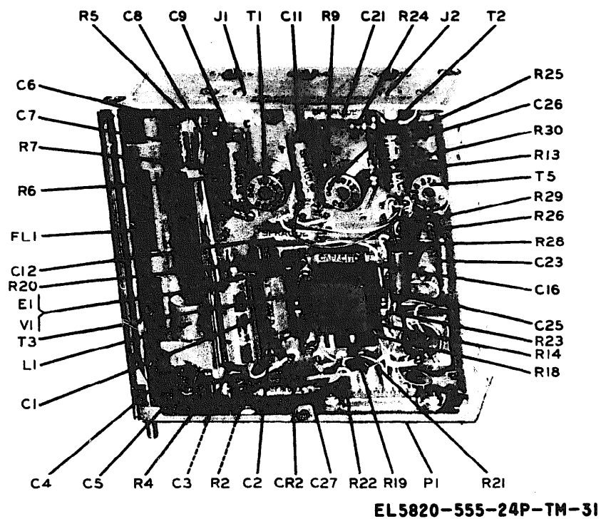
Figure 3-31. AM i-fla-f amplifier module, front view, cover removed (1A5A6).
