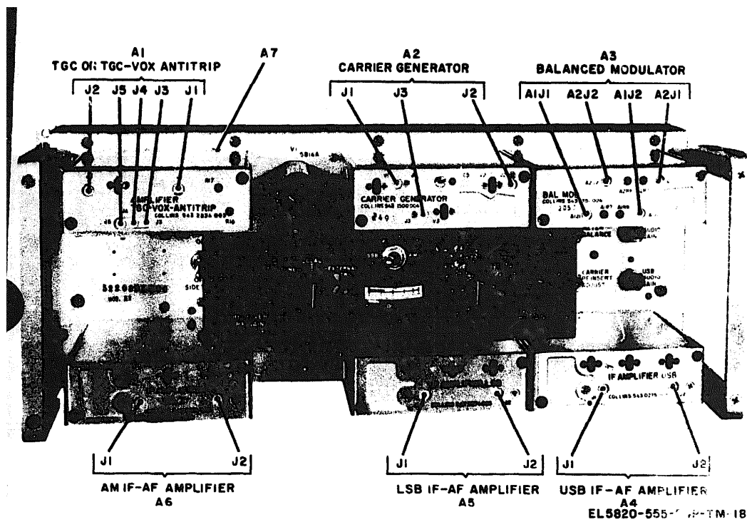
Figure 3-18. Sideband Generator 786F-1, module location (145).
