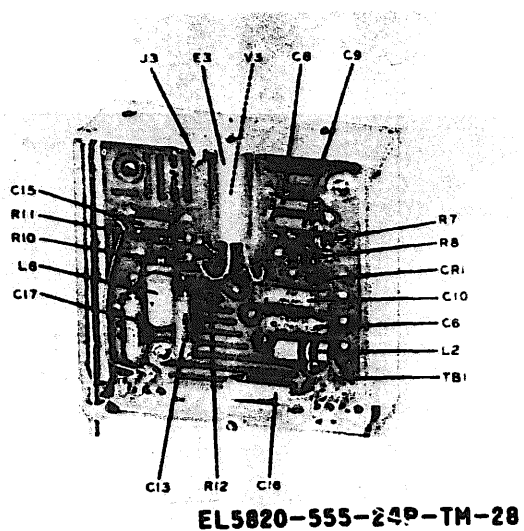
Figure 3-28. Carrier generator module, front view, cover removed (1A5A2).
