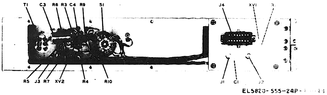
Figure 3-48. Frequency Comparator CM-126/UR, rear view, cover removed (1A8).
