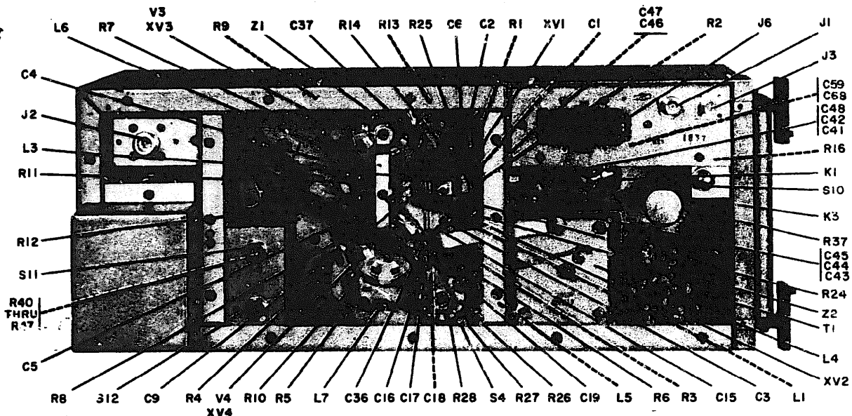
Figure 3-38. Power Amplifier 367A-3, rear view, cover removed (1A3).
