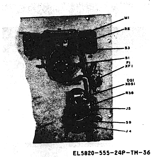
Figure 3-36. Power Amplifier 367A-3, front panel, rear view (1A3).
