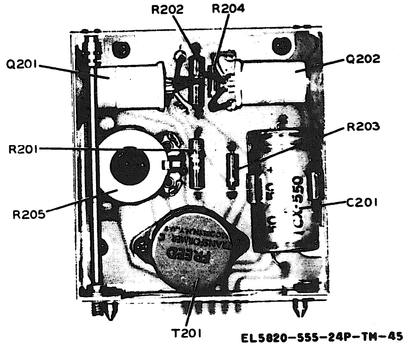
Figure 3-45. Speaker amplifier module, component side (1A7A7).
