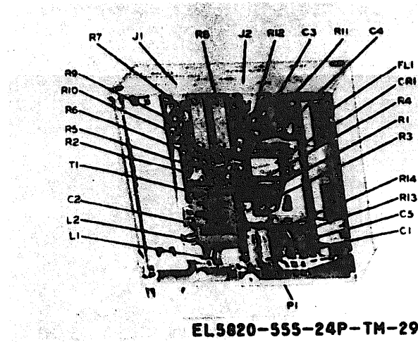
Figure 3-29. Balanced modulator module, usb modulator assembly, cover removed (1A5ASA1).
