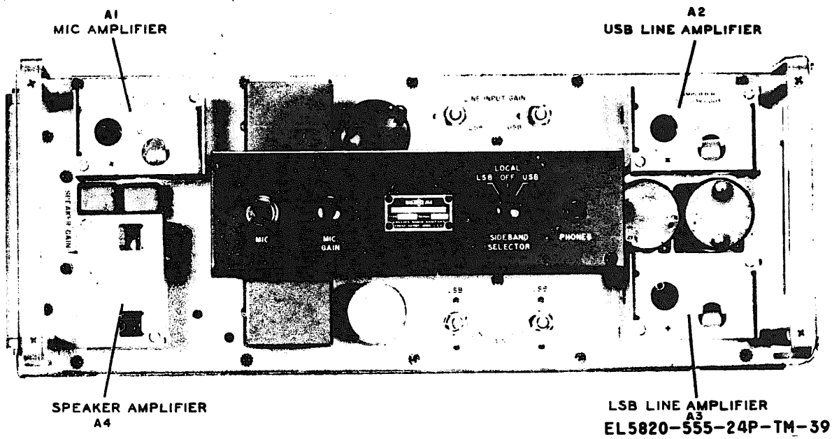
Figure 3-39. Audio and Control Unit 159B-1, module location (1A7).
