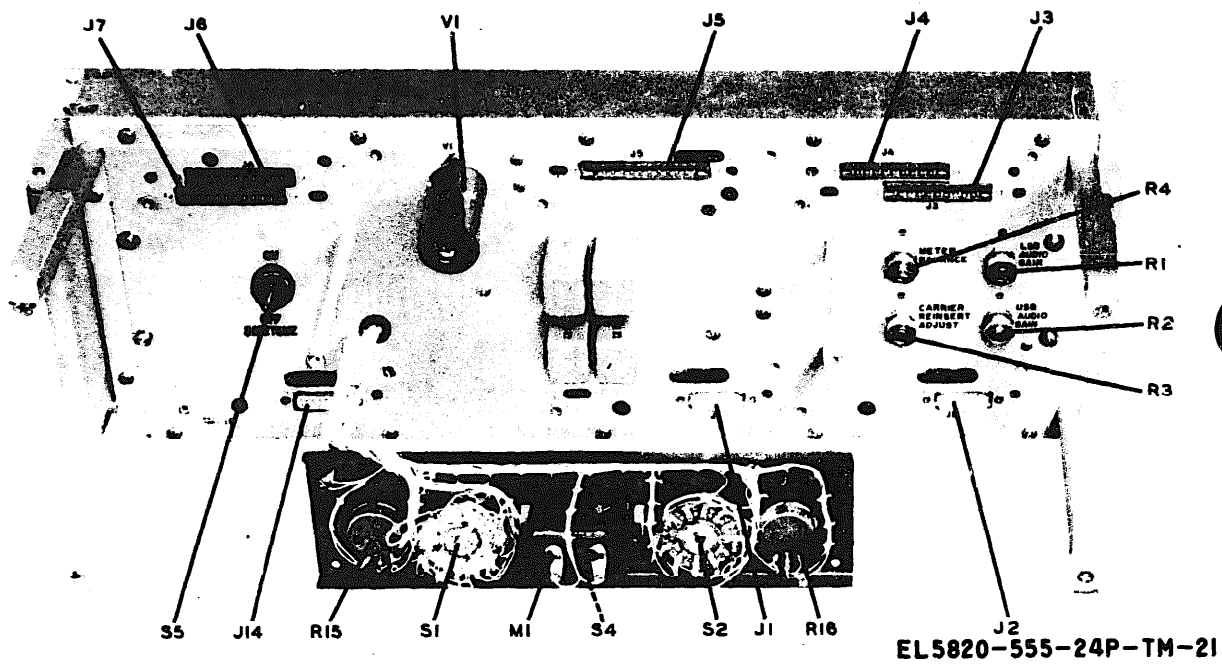
Figure 3-21. Sideband Generator 786F-1 chassis, front view (1A5A7).
