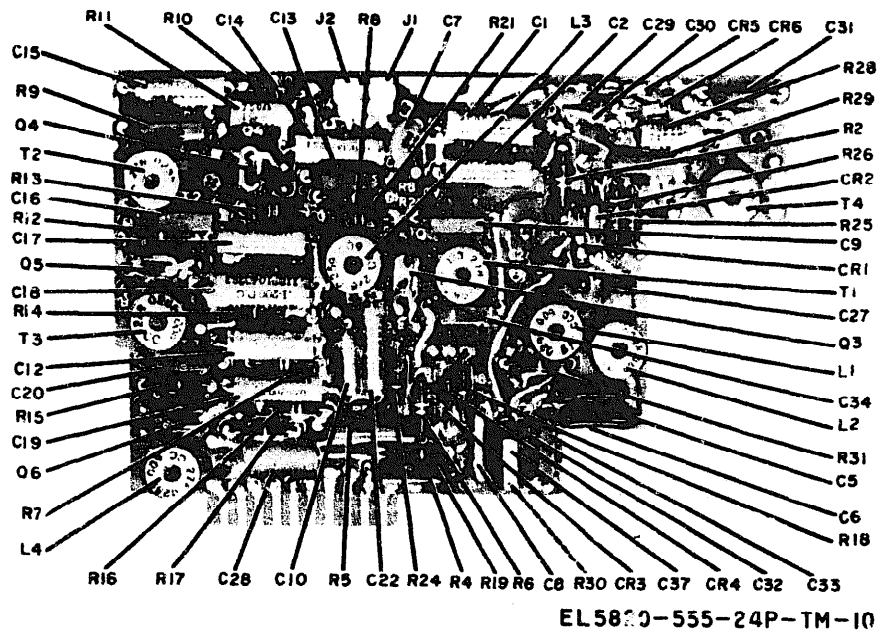
Figure 3-10. Stabilized Master Oscillator, Model B, i-f amplifier board (1A4A3A2).
