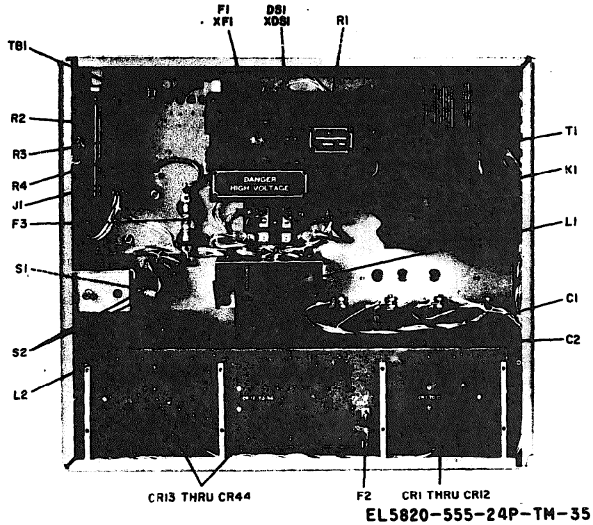
Figure 3-35. High-Voltage Power Supply PP-2153/U, front view, cover removed (1A12).
