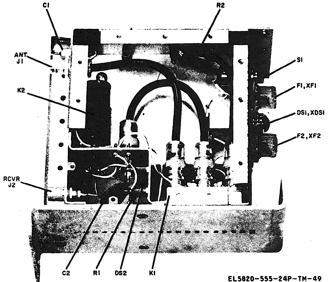
Figure 3-49. Thermal relay input portector, bottom view, cover removed (1A1).
