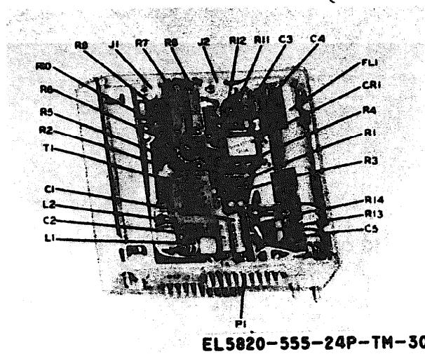
Figure 3-30. Balanced modulator module, Isb modulator assembly, cover removed (1A5ASA2).
