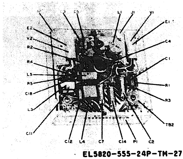
Figure 3-27. Carrier generator module, front view, cover removed (1A5A2).
