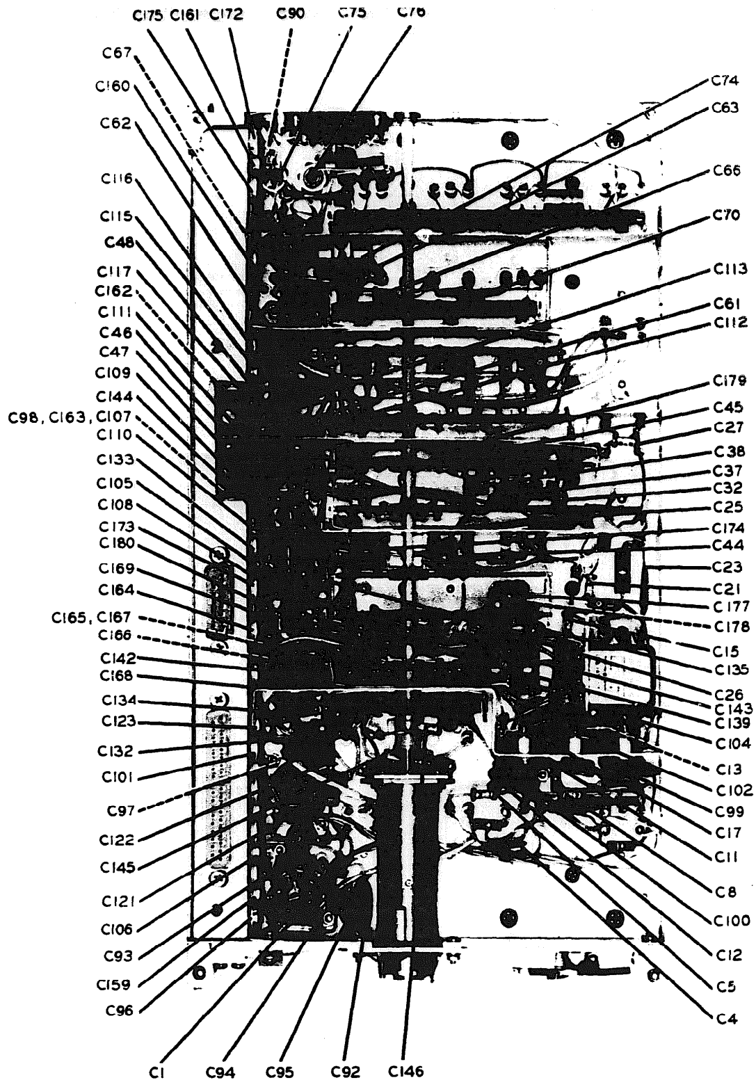
Figure 3-15. R-F tuner module, capacitor location (1A4A4).
