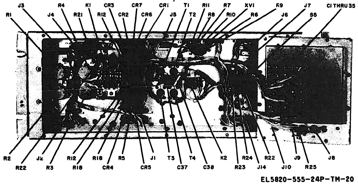
Figure 3-20. Sideband Generator 786F-1 chassis, rear view, cover removed (1A5A7).
