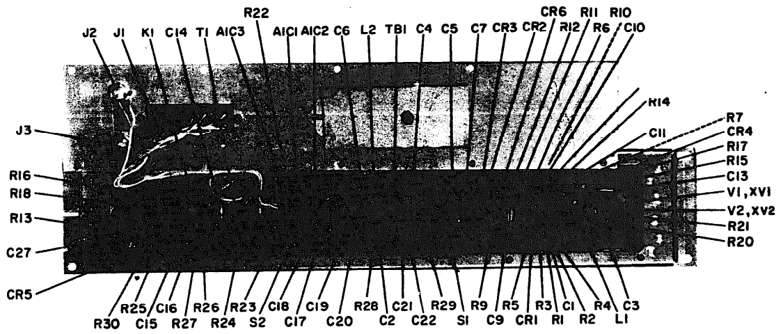
Figure 3-53. CW and fsk unit, rear view, cover removed (1A6).
