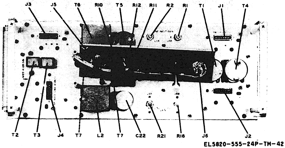
Figure 3-42. Audio and Control Unit 159B-1 chassis, front view (1A7).
